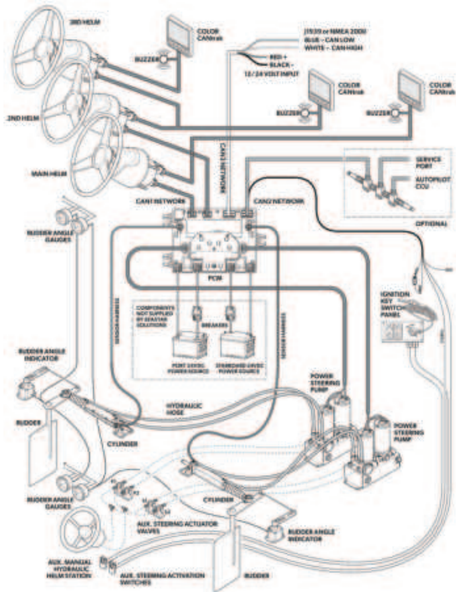
Example of twin rudder system schematic.
