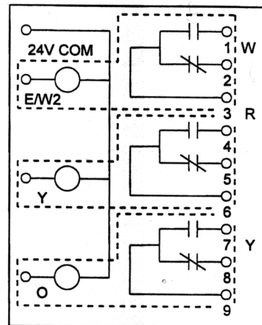
MODEL 8024 SCHEMATIC
