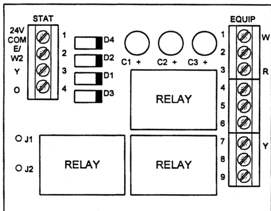
MODEL 8024 LAYOUT
