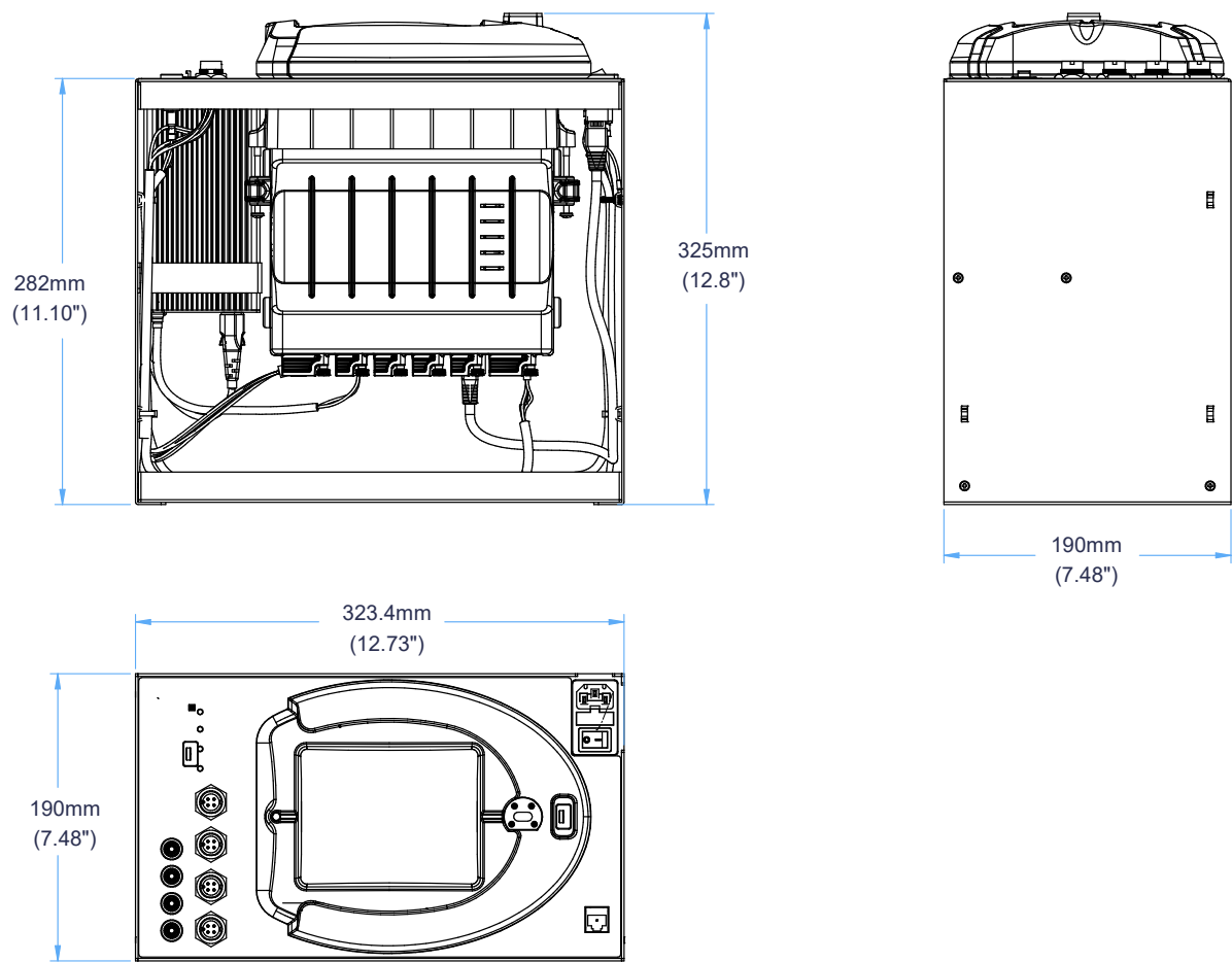
Figure 4: Device Dimensions
