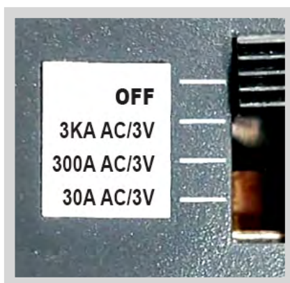
Figure 3: Rated-current Switch
