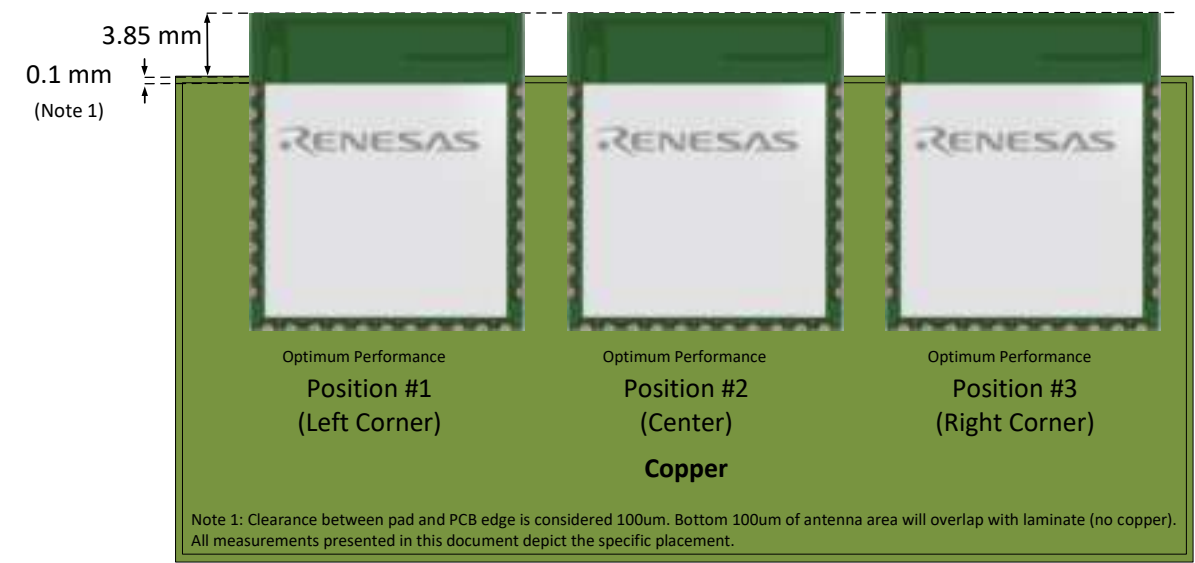
Figure 7. Installation locations for optimum antenna performance
