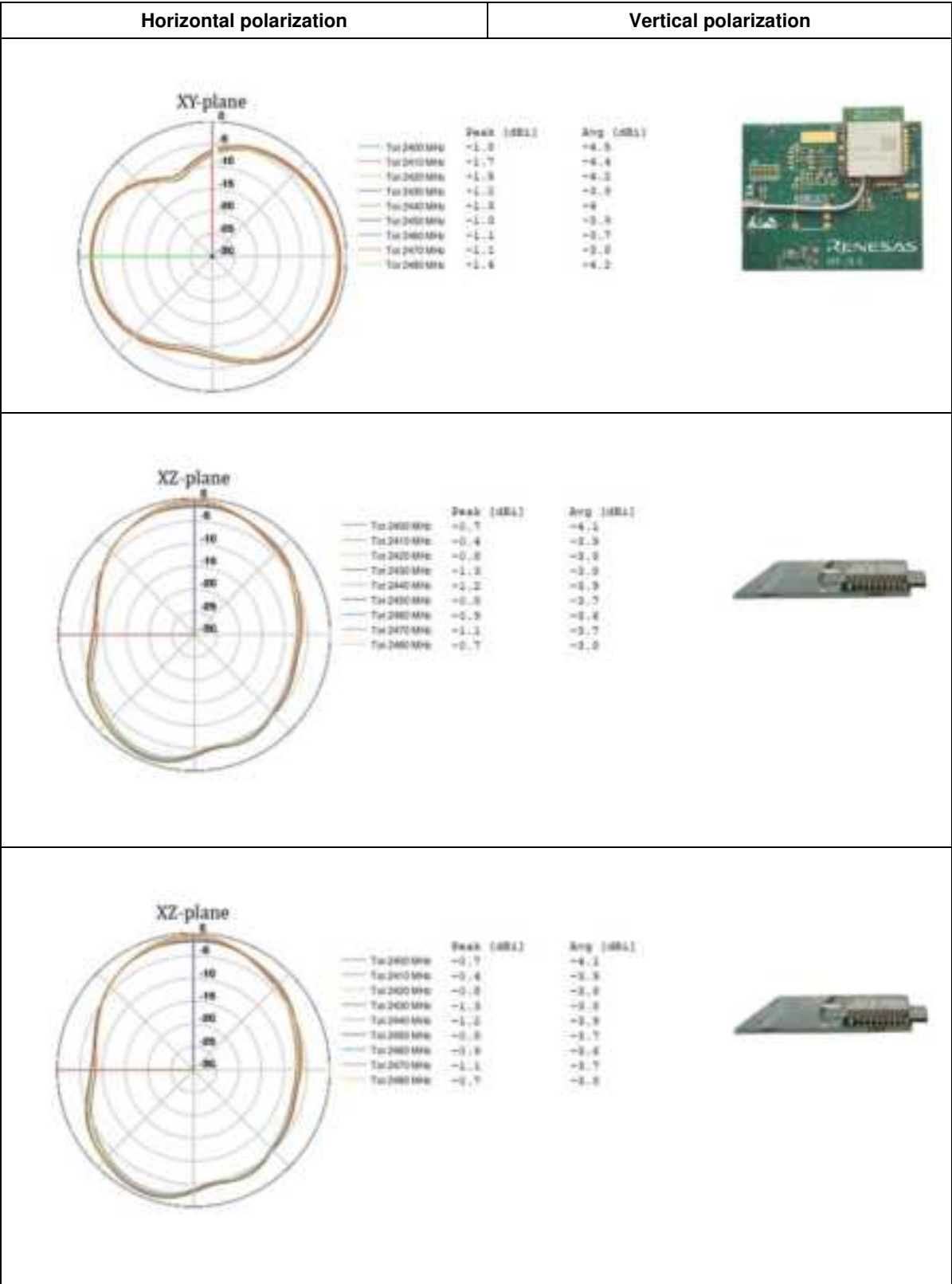
Figure 15. Radiation pattern for trace antenna
