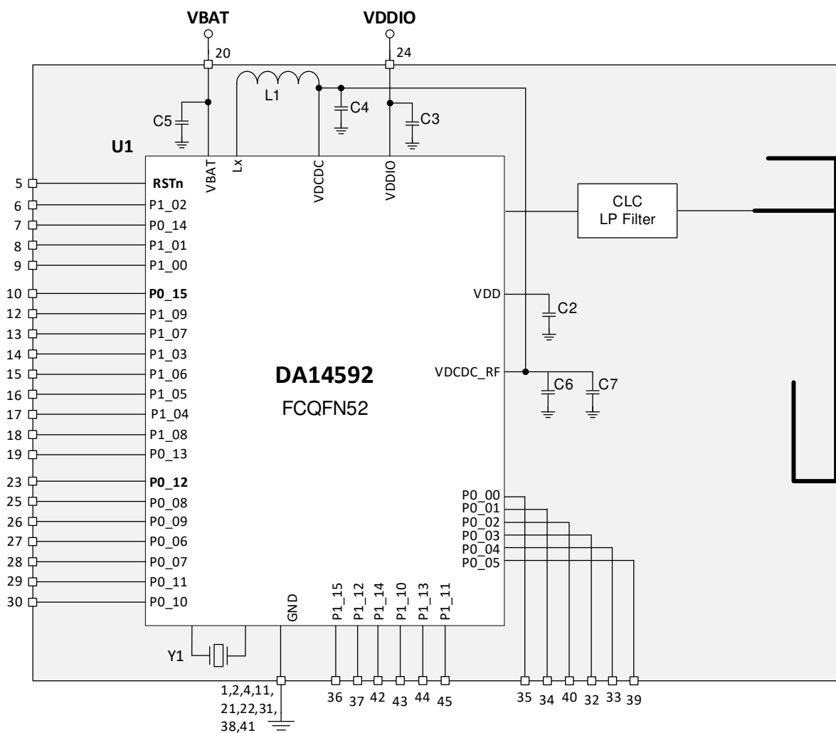
Figure 1. DA14592MOD-0100000 block diagram
