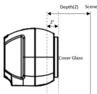
Gemini 335L/336L Depth Start Point
