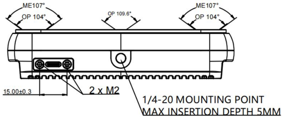
Gemini 335L Product Drawing Bottom View
