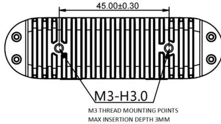
Gemini 336 Product Drawing Rear View
