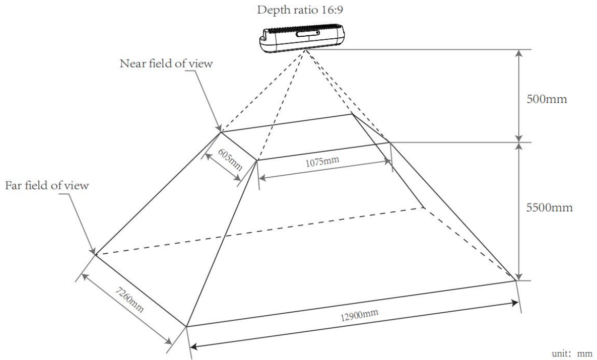
Gemini 335L/336L Depth FOV for Aspect Ratio = 16:9
