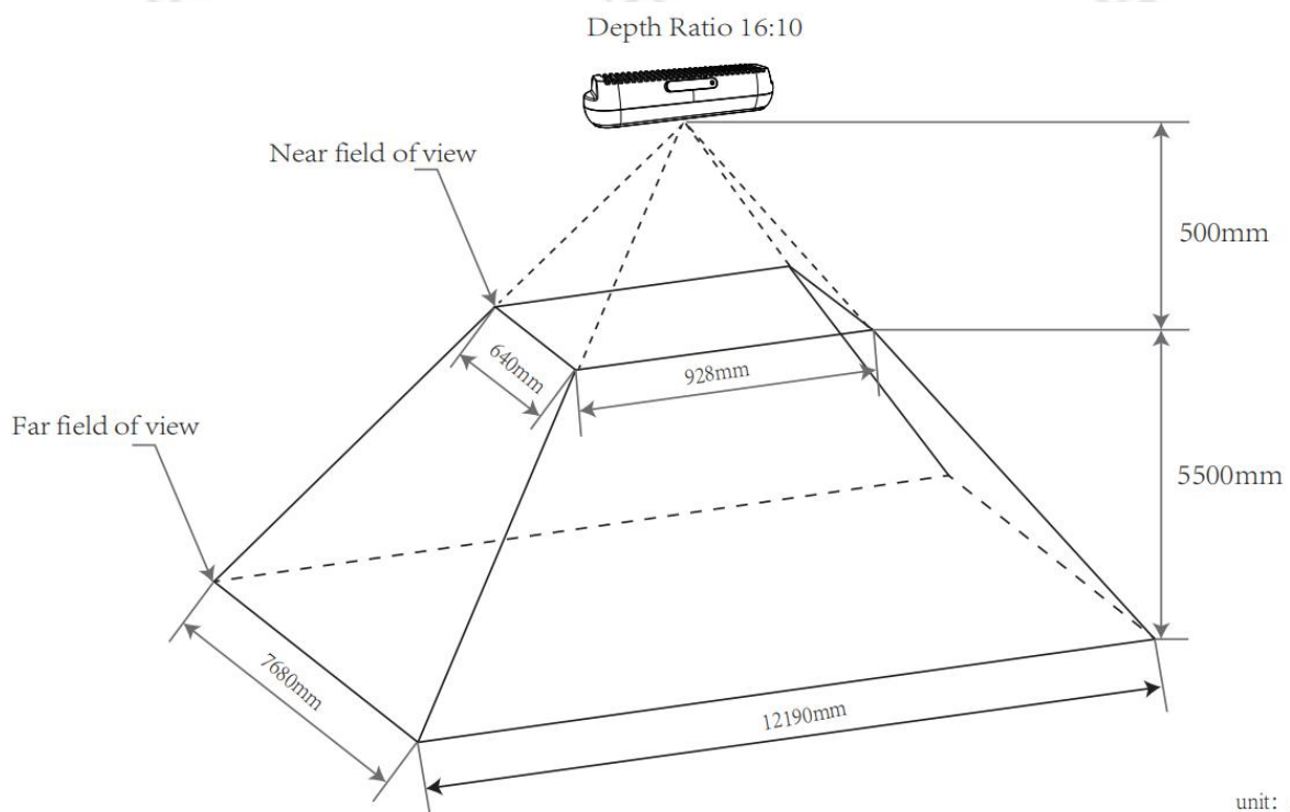
Gemini 335L/336L Depth FOV for Aspect Ratio = 16:10
