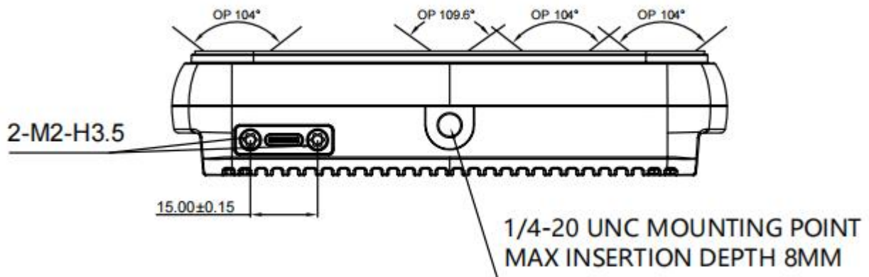
Gemini 336L Product Drawing Bottom View
