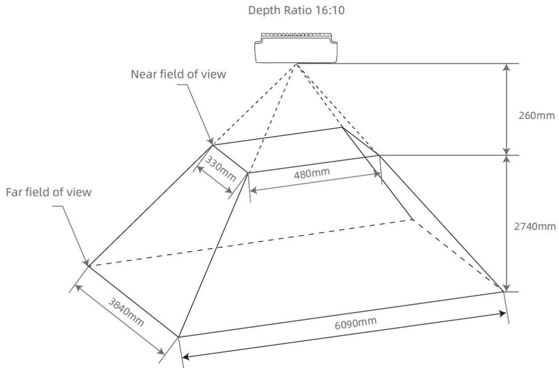
Gemini 335/336 Depth FOV for Aspect Ratio = 16:10
