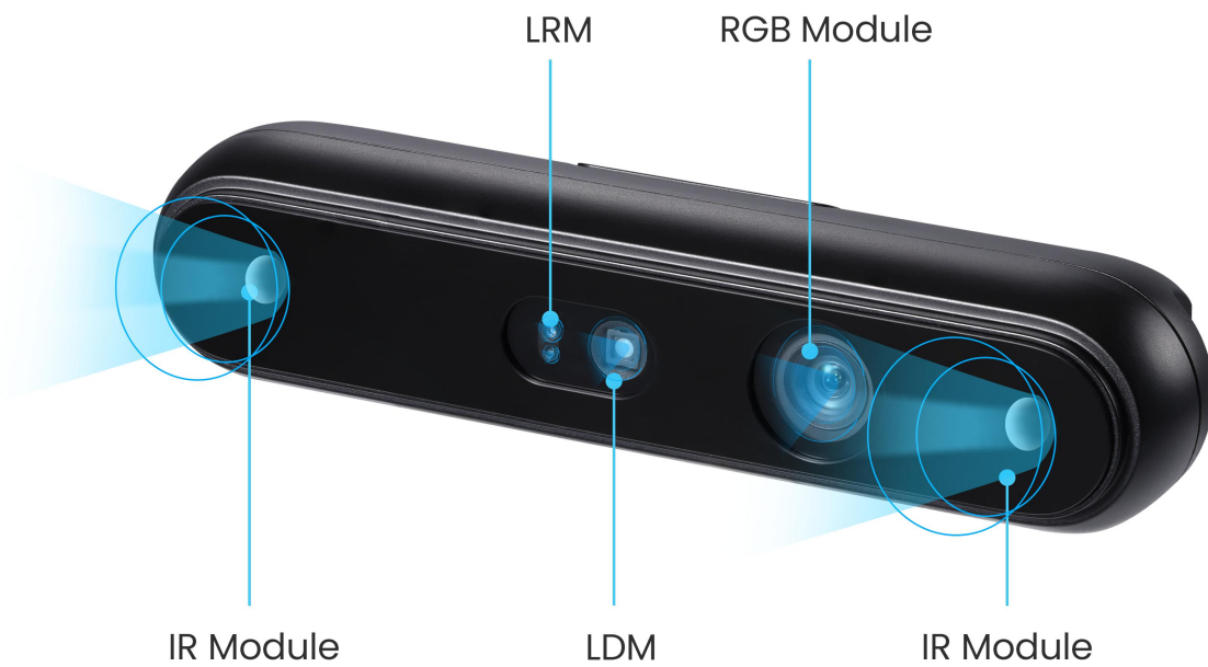
Gemini 336L Components
