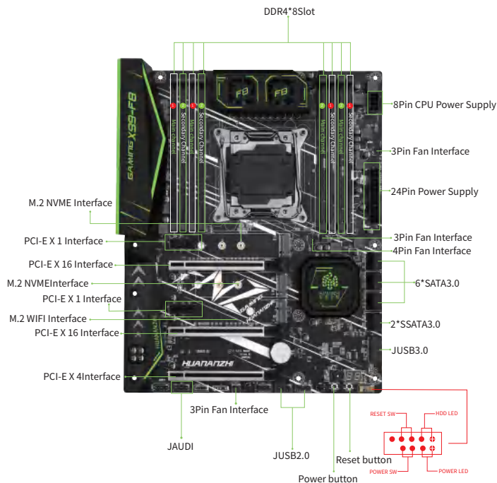
1-1 X99-F8 Motherboard Illustration
