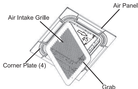
Fig. 2.1 Removing Method of Air Intake Grille
