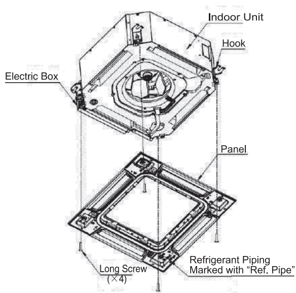
Fig. 2.3 Installation
