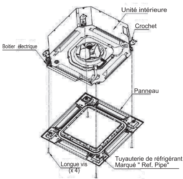
Fig. 2.3 Installation
