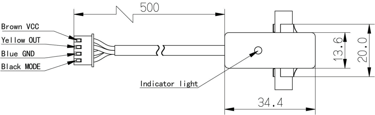
9th.Y26A wiring diagram of various models
