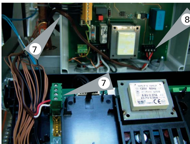
Fig. 8 Boiler Power Pump Module (WB1A shown)
