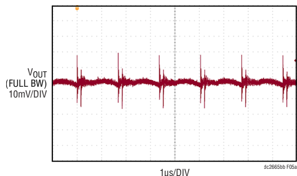
(a) 1V_{OUT} , 600kHz, Full Bandwidth at 500MHz
