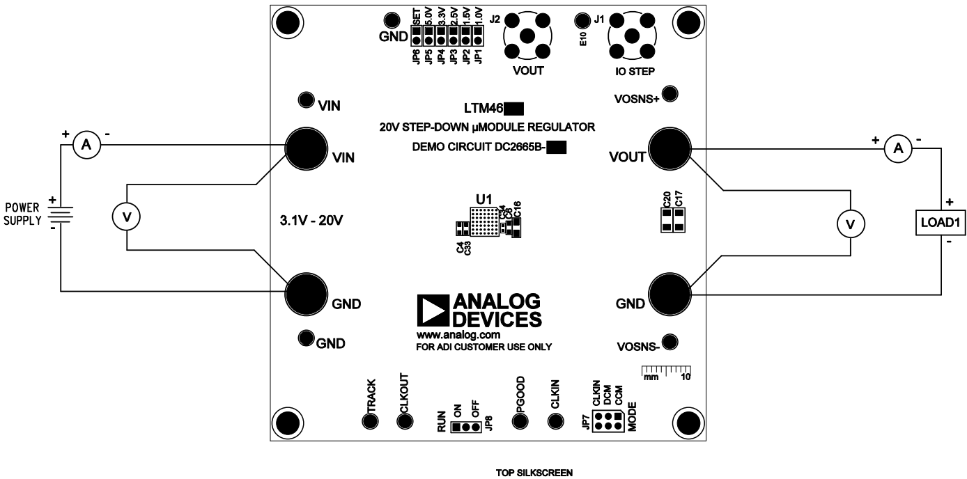
Figure 1. Test Setup of DC2665B-B
