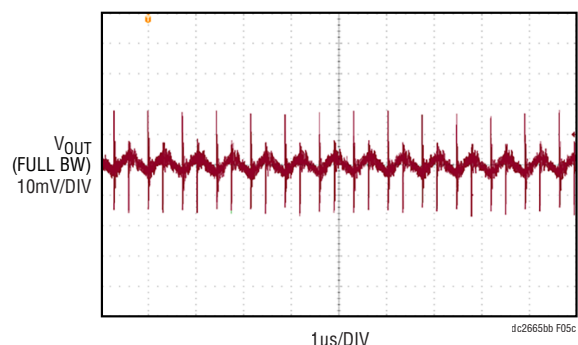
(c) 5V_{OUT} , 1.5MHz, Full Bandwidth at 500MHz
