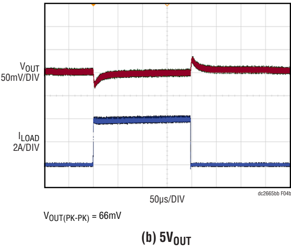
Figure 4. Load Transient (7.5A to 11.25A) Response Waveform at 12VIN
