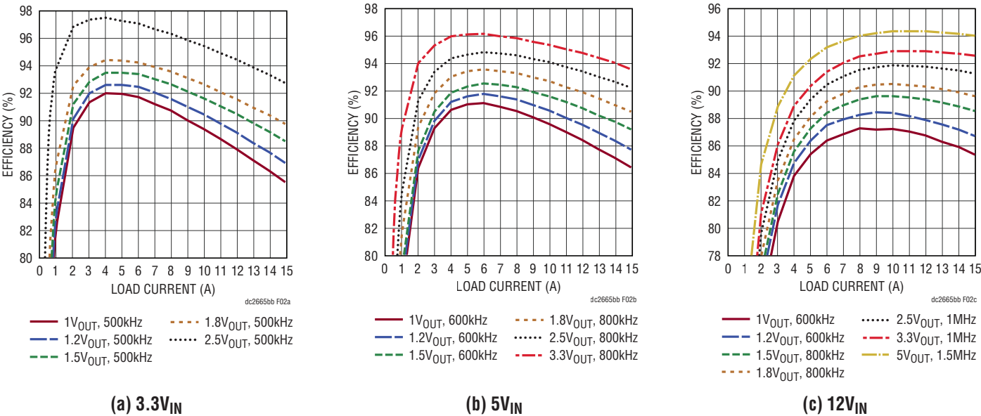
Figure 2. Measured Supply, CCM Efficiency vs Load Current
