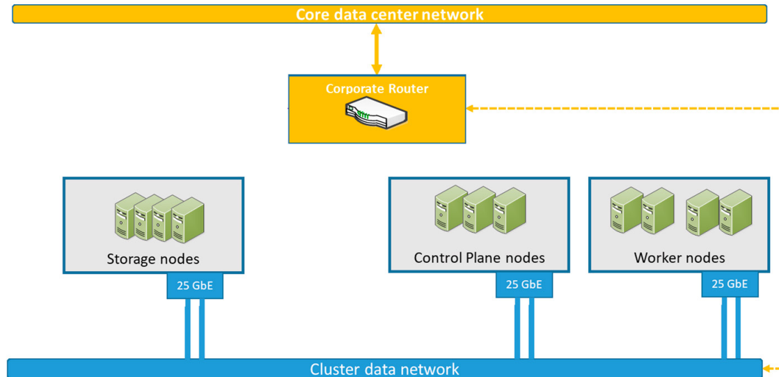
Figure 9. Physical network infrastructure
