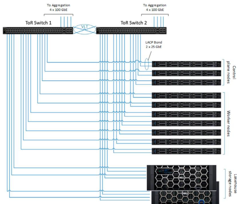
Figure 10. Cluster data network connections
