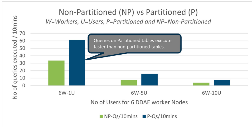
Figure 11. Number of TPC-DS queries executed every 10 minutes against Partitioned and non-partitioned 1TB (SF1K) Dataset.
