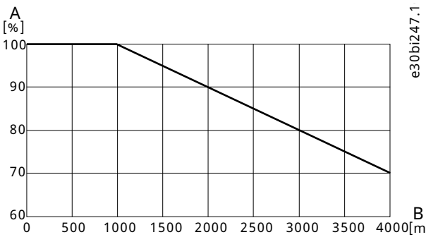
Figure 104: Output Current Derating vs. Installation Altitude
