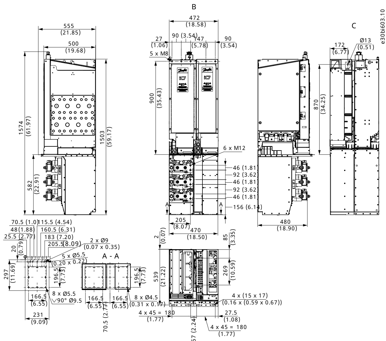
Figure 73: Dimensions of the LCL Filter and the AFE Module with the Standard Integration Unit in mm (in), AR11
