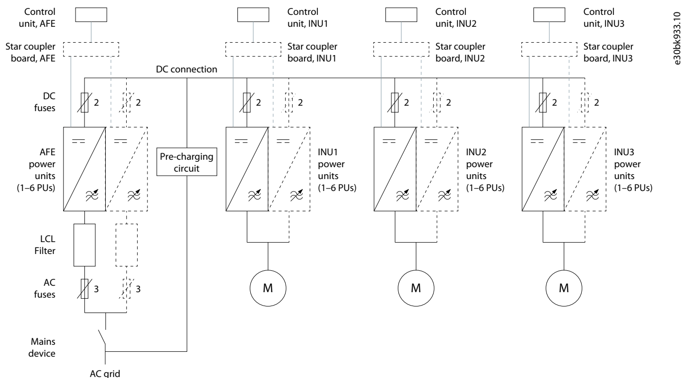
Figure 29: DC Connections of a Drive Lineup
