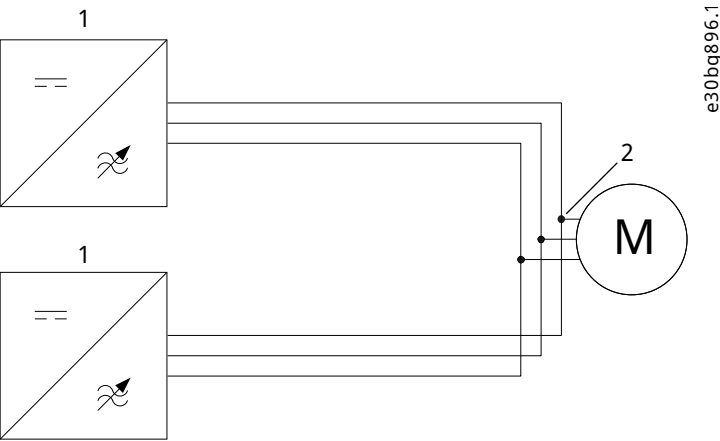
Figure 19: Recommended Installation
