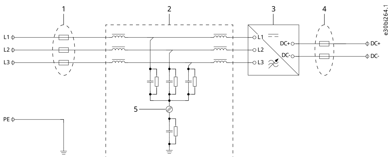
Figure 24: Diagram of the LCL Filter
