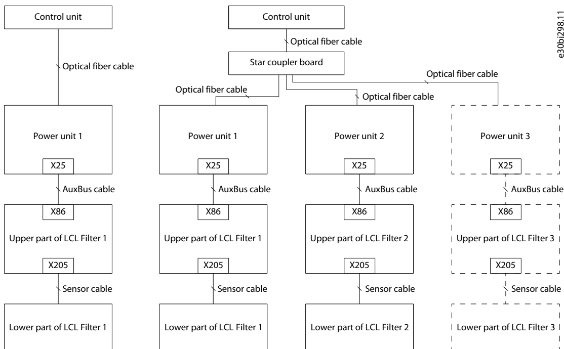
Figure 33: AuxBus Topology for AFE Modules and LCL Filters
