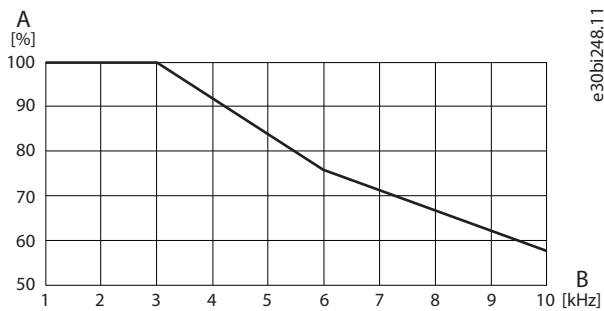
Figure 105: Output Current Derating vs. Switching Frequency (INU)
