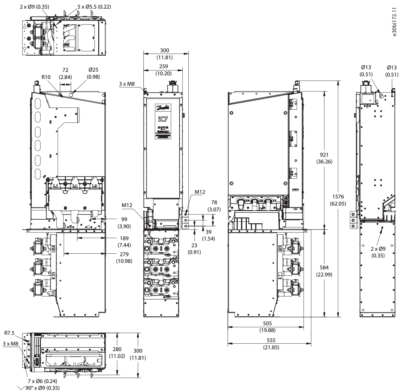
Figure 75: Dimensions of the LCL Filter in mm (in), Size 10 and 11
