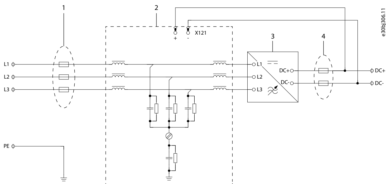
Figure 22: Diagram of the LCL Filter Fan Supply
