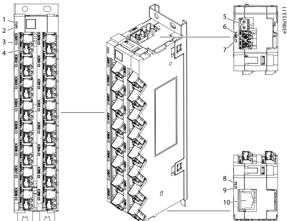
Figure 42: The Star Coupler Board with 16 Ports
