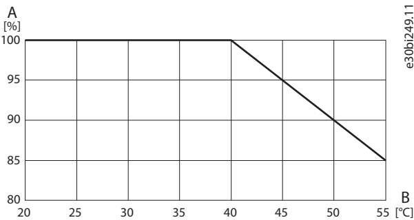
Figure 103: Output Current Derating vs. Ambient Temperature
