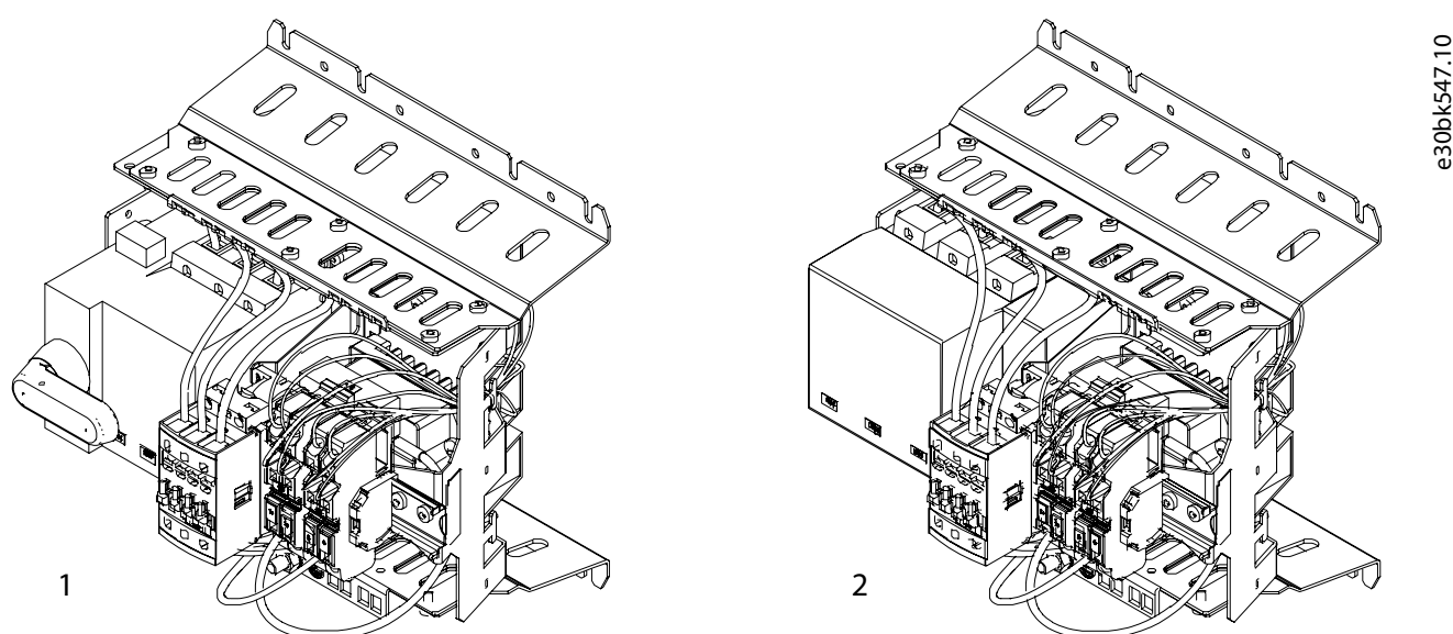
Figure 38: Pre-charging Units
