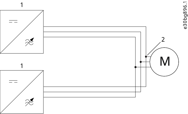
Figure 19: Recommended Installation
