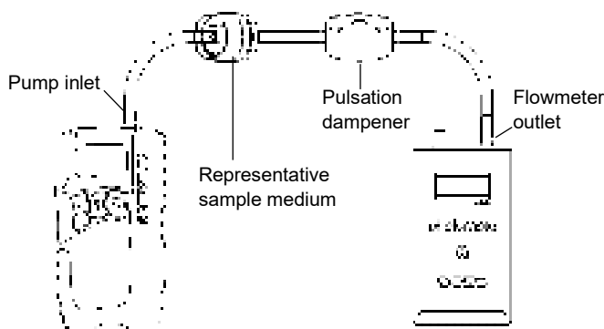
Figure 3. High Flow Rate Verification Train
