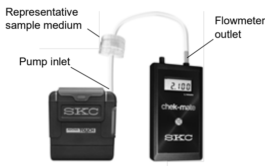
Figure 2. Medium and Low Flow Rate Verification Train (Medium Flow Pump and Flowmeter Shown)
