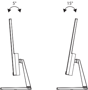
Tilting angle -5° (±2.0°) - +15° (±2.0°)
