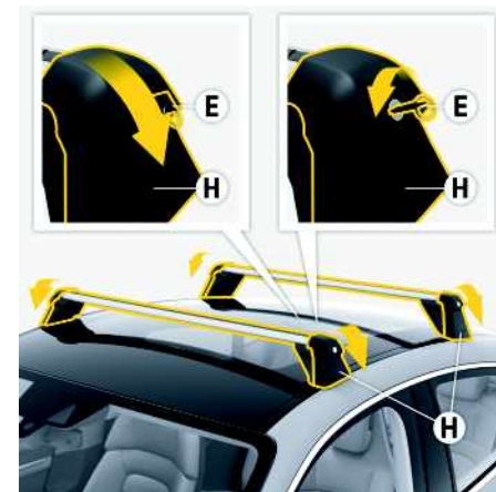
Fig. 171: Fold down the cover flaps and lock
