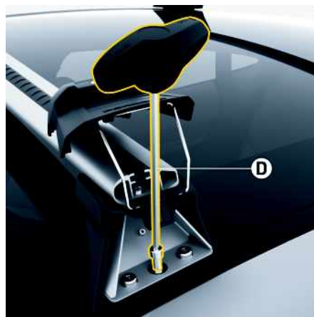
Fig. 170: Tighten fastening screws.
