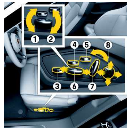
Fig. 180: Adjusting an electric seat
