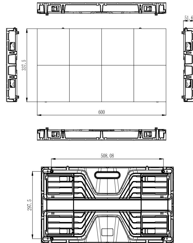
Cabinet dimensions
