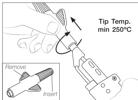
Through-Hole Desoldering
