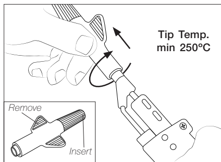
Through-Hole Desoldering
