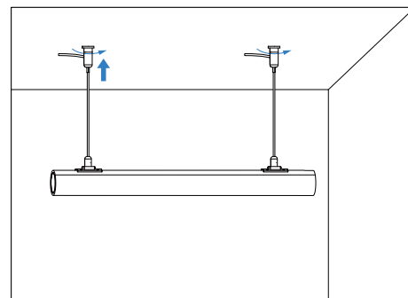
6 Spin upwards to the limit
