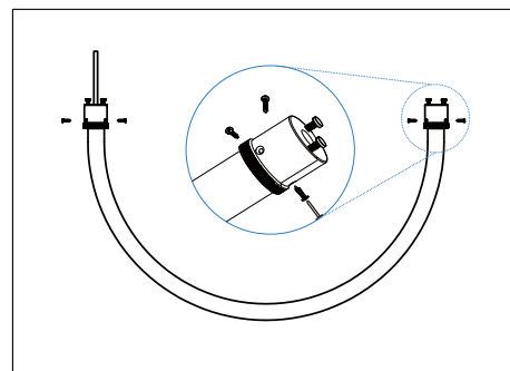
3 Put accessories into the tube and fix with screws
