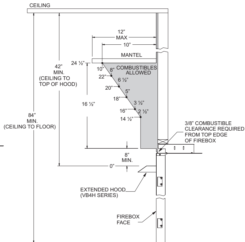
Figure 3b - Mantel Clearances with Optional Extended Hood
