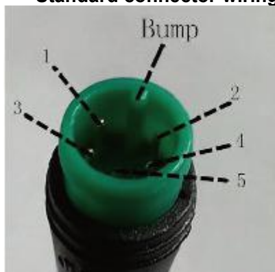
Display-side connector
