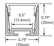
DUET-04-CHAN-XXX-6.5 XXX = SLV (silver), WHT (white), GLD (gold), BLK (black) Aluminum extrusion
