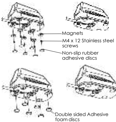
Optional magnetic base kit
