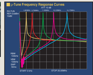
10 dB/Div • 2 MHz/Div
