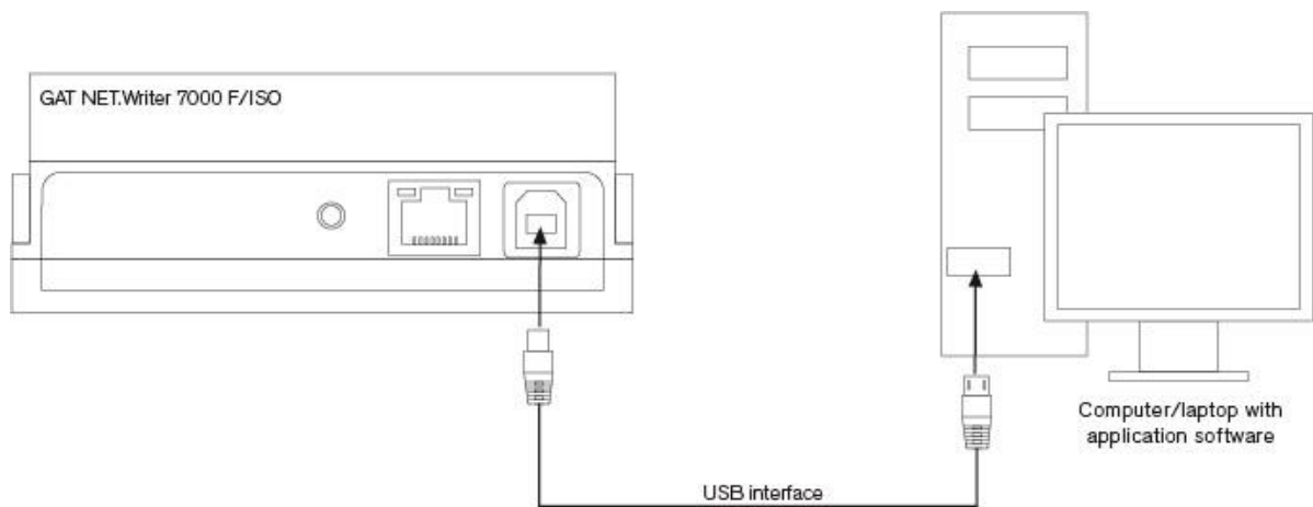
Figure 3.1 – USB connection
