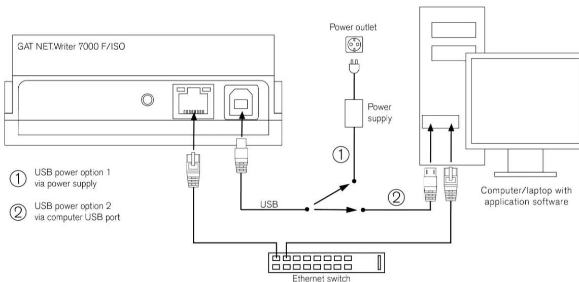
Figure 3.2 – Ethernet connection
