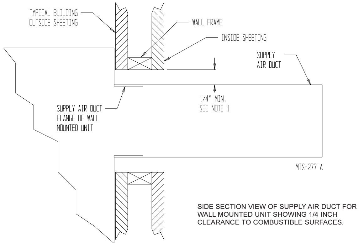
FIGURE 4 ELECTRIC HEAT CLEARANCE W30A1, W30L1, W36A1, W36L1, W42A1, W42L1, W48A1, W48L1, W60A1, W60L1
