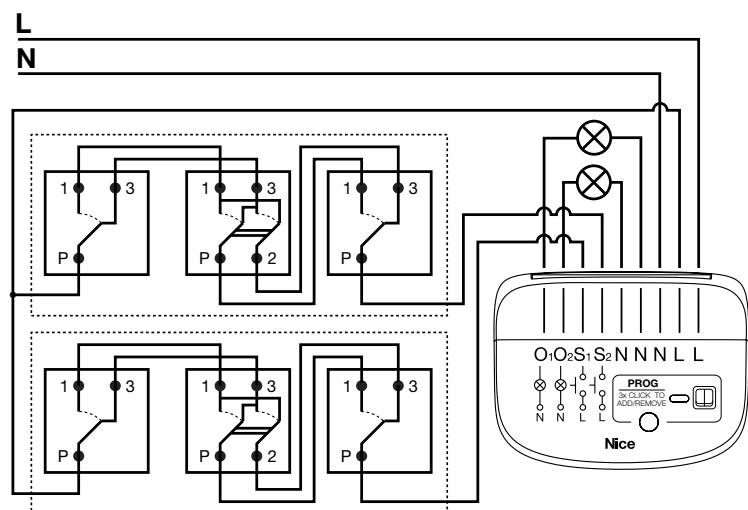
Figure 6: Stair-cross switches ×2
