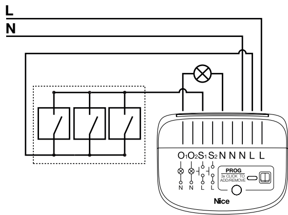
Figure 3: Momentary switches ×1
