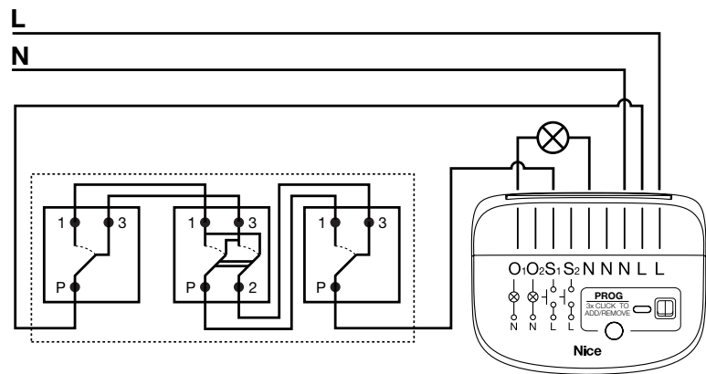
Figure 5: Stair-cross switches ×1
