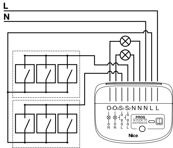
Figure 4: Momentary switches ×2
