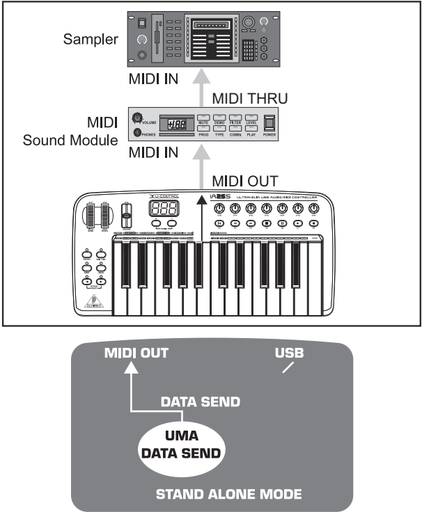
Fig. 1.4: Stand-alone mode
