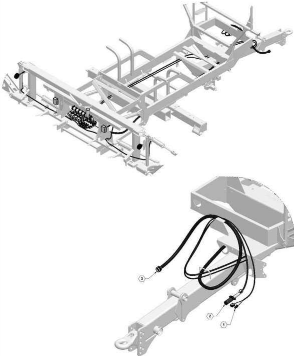
9613TF-80 HARNESS I.D. &amp; LOCATION
