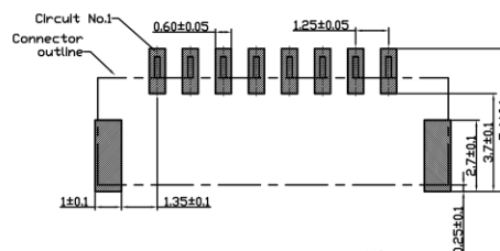
GH-nAWB \frac{\text{PCB寸法}}{\text{PCB Layout}}
