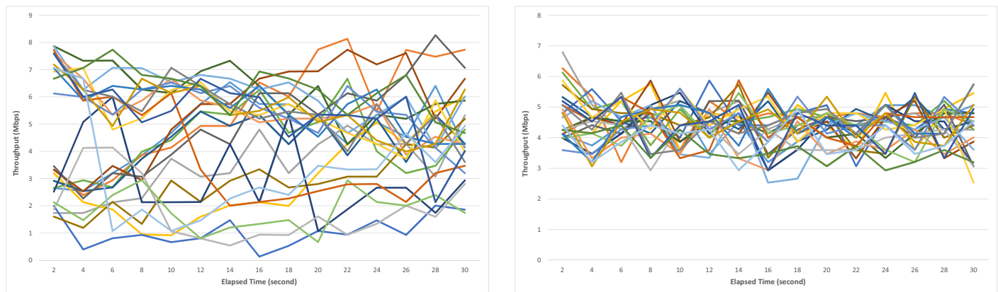
Figure EC3-7 Effect of Airtime Fairness Algorithm on Individual Flows
