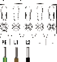
IT/TT 1-phase (230V)
