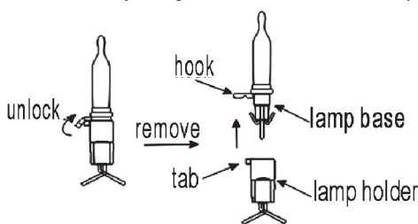
Fig. 1 Unlock and remove the burned out lamp
