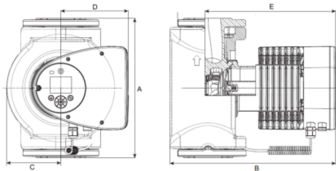
Figure 23: Grundfos Variable Speed Pump Dimensions
