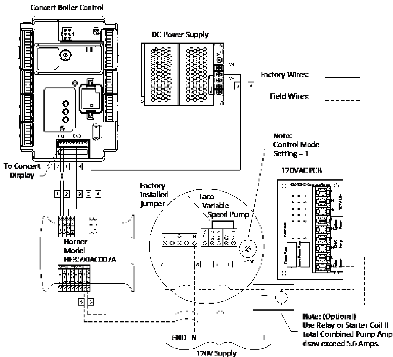
Figure 8: Taco Variable Speed Pump Wiring Schematic
