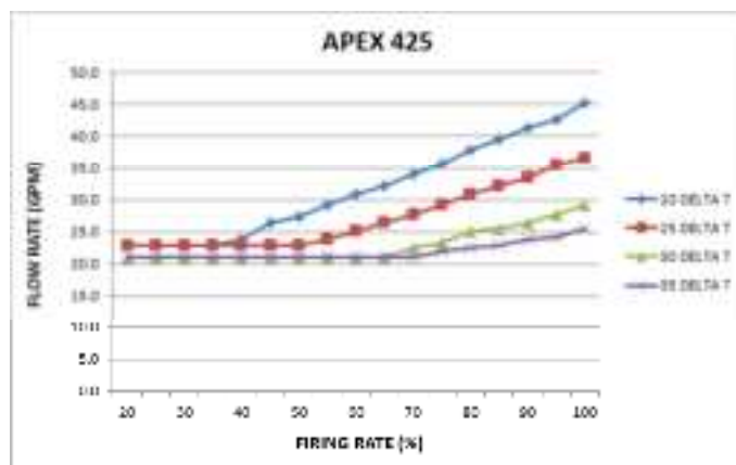
Figure 3: Pump Flow vs. Firing Rate
