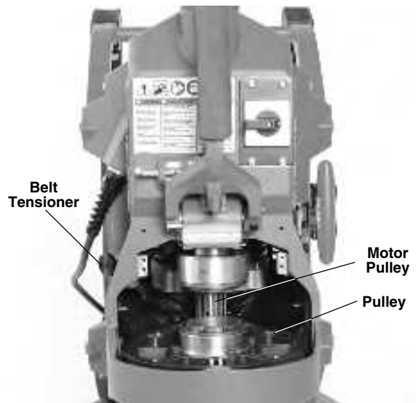
Figure 19 – Machine Standing on Back, Drip Tray Removed
