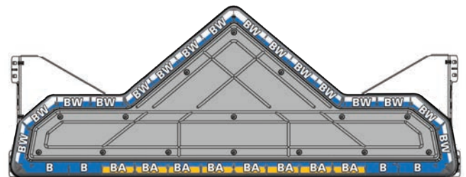
VALR51J-P2L (without interface module, low hook mount)
