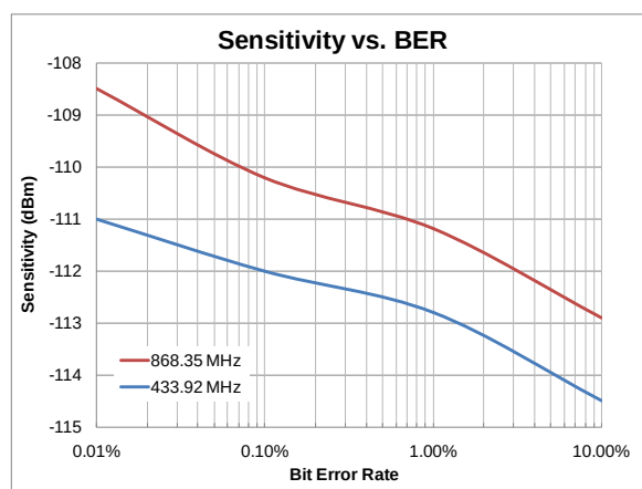
Figure 8. Sensitivity vs. BER, F_{RF} = 433.92 / 868.35 MHz, V_{DD} = 3.3 V, SR = 1 kps
