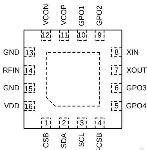
Figure 2. CMT2219A Pin Assignments
