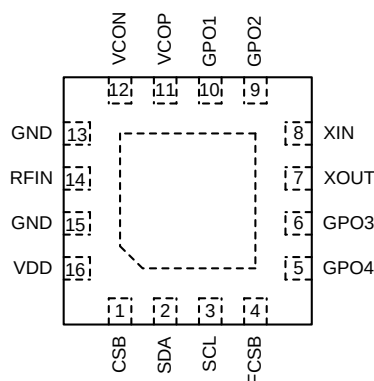
CMT2219A Top View
