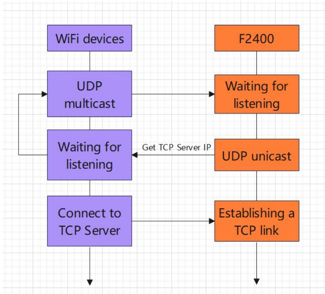
Diagram of LAN Device Discovery
