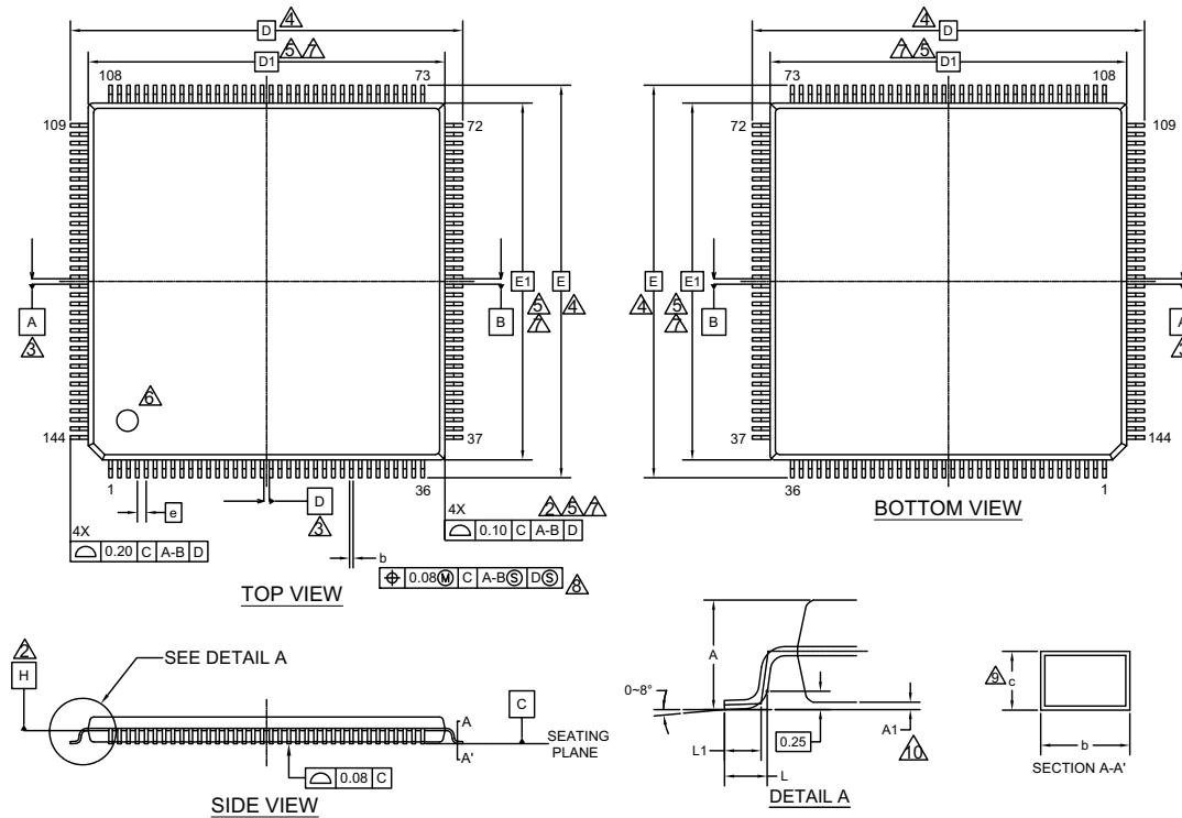
Figure 28-2.144-LQFP Package Outline
