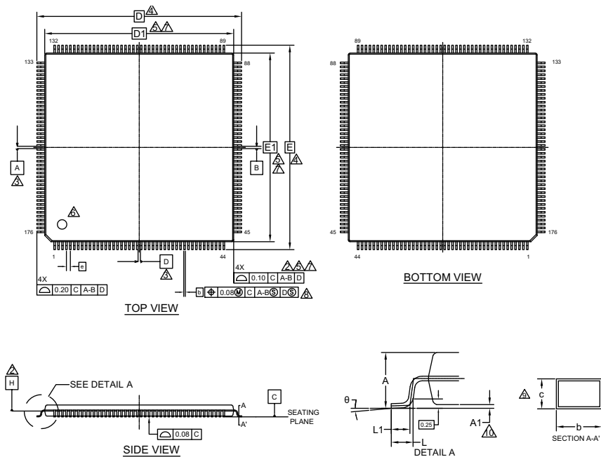
Figure 28-1.176-LQFP Package Outline
