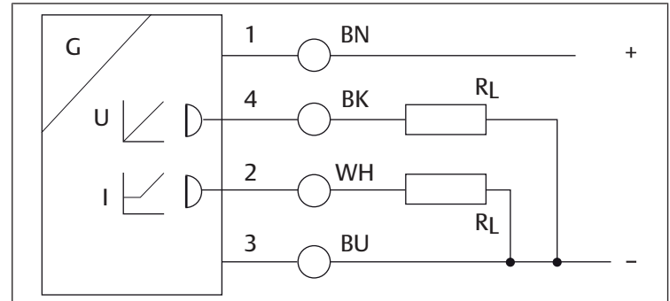
Fig. 3: Plug assignment
