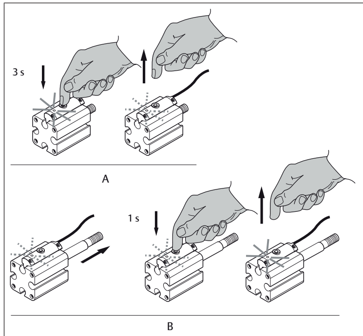
Fig. 5: Teaching in zero point (A) / teaching in end point (B)
