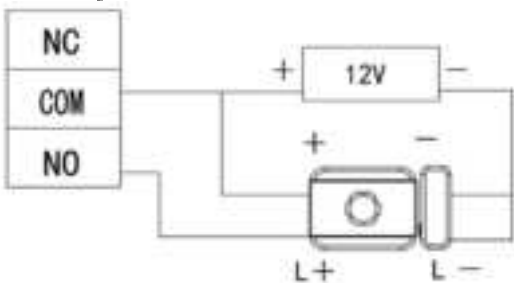
Figure 2-6 Electric lock
