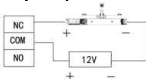
Figure 2-8 Electric bolt
