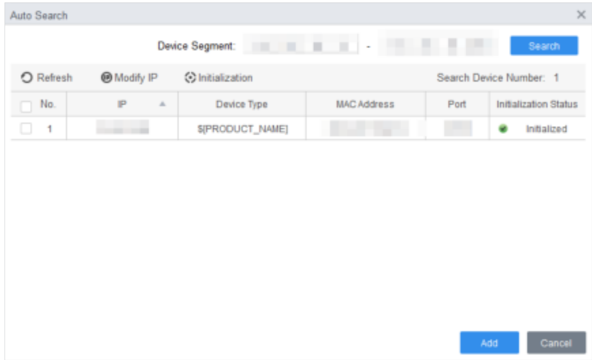
Figure 3-5 Auto search
