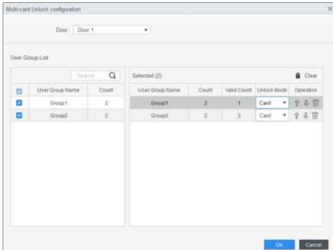
Figure 3-20 Multi-card unlock configuration (2)
