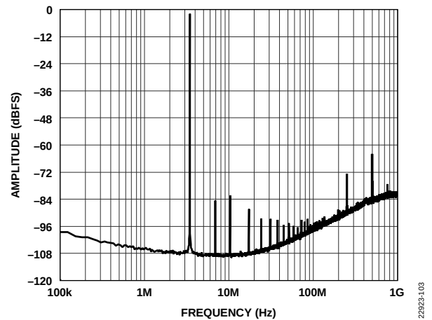
Figure 7. ADC Noise Floor at Backoff = 3 dB, 2 GSPS
