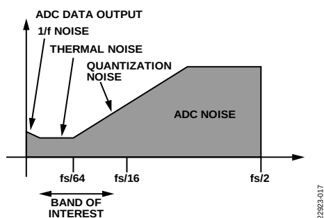
Figure 54. Noise Regions of a \Sigma - \Delta ADC
