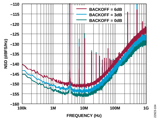
Figure 8. ADC NSD at Various Backoff Values, 2 GSPS
