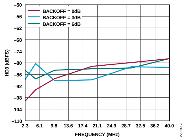
Figure 27. ADC HD3 vs. Frequency at Various Backoff Values and A_{IN} = -10 dB, 2 GSPS
