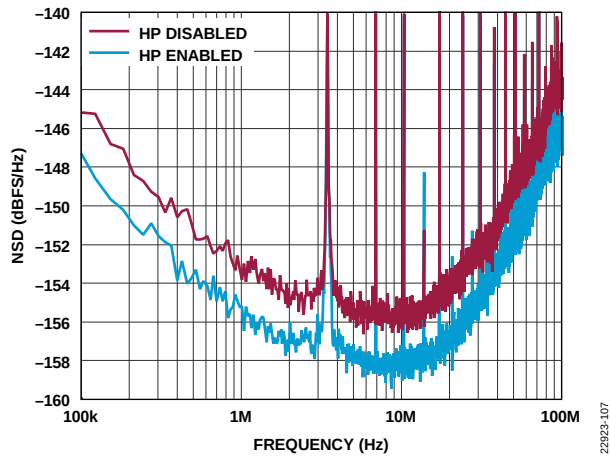
Figure 11. ADC NSD with and Without EN_HP, 2 GSPS
