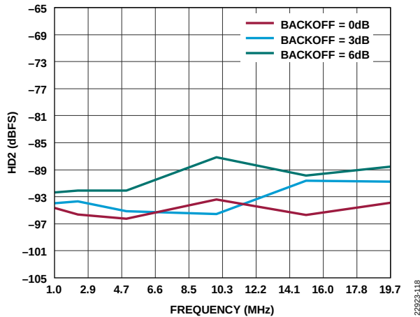
Figure 22. ADC HD2 vs. Frequency at Various Backoff Values and A_{IN} = -10 dB, 1 GSPS
