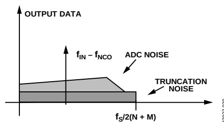
Figure 75. Example Showing ADC Noise Unaffected by Truncation Error
