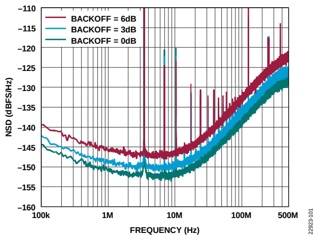
Figure 5. ADC NSD at Various Backoff Values, 1 GSPS
