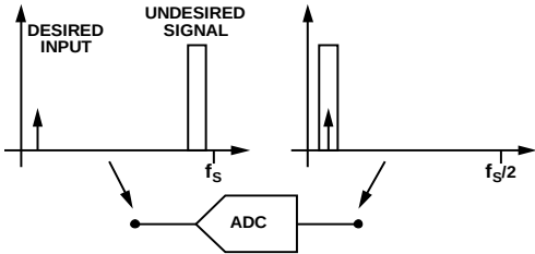
Figure 62. Aliasing in a Discrete Time ADC
