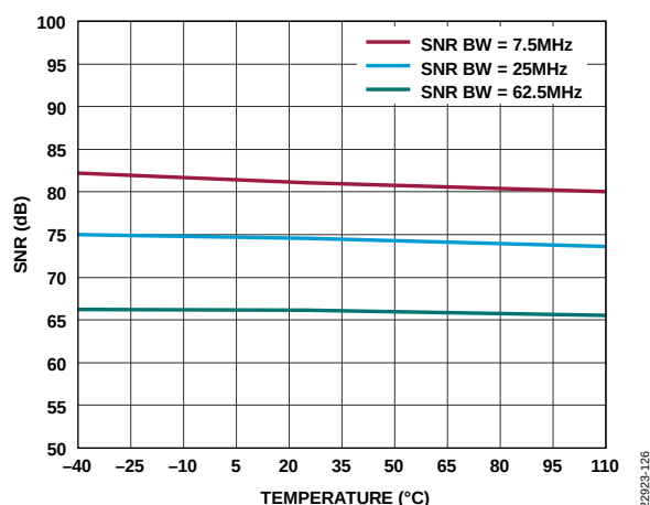
Figure 30. ADC SNR vs. Junction Temperature, 1 GSPS
