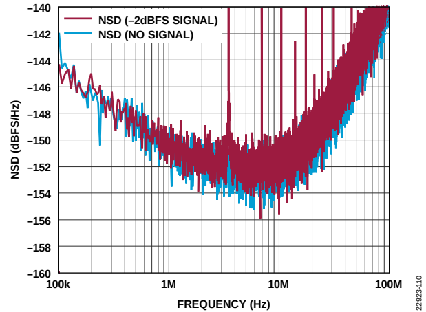
Figure 14. ADC NSD with and Without Full-Scale Input Signal, 1 GSPS
