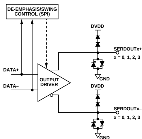
Figure 51. Digital Outputs
