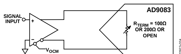
Figure 61. DC-Coupled Inputs to the AD9083 Using an Amplifier (Note the V_{OCM} Pin Providing the Common-Mode Voltage)
