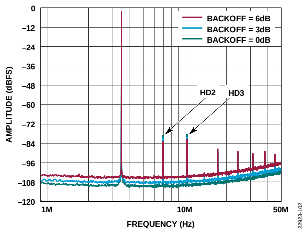
Figure 6. Harmonic Distortion 2 (HD2) and Harmonic Distortion 3 (HD3) at Various Backoff Values, 1 GSPS
