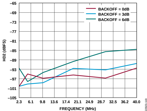
Figure 23. ADC HD2 vs. Frequency at Various Backoff Values and A_{IN} = -10 dB, 2 GSPS
