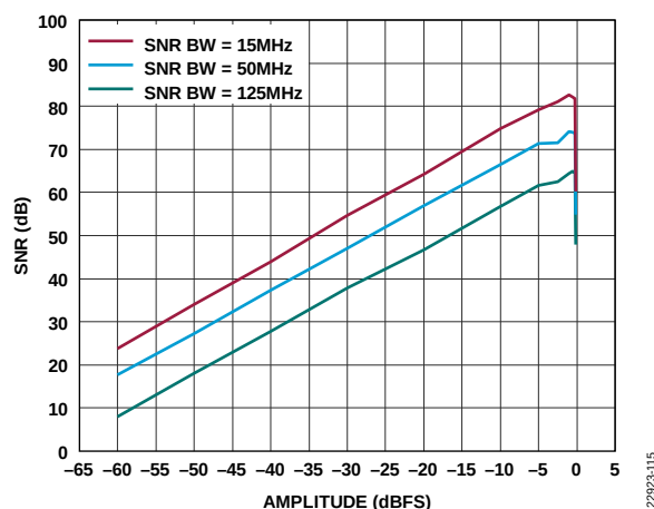
Figure 19. ADC SNR vs. Input Amplitude, 2 GSPS
