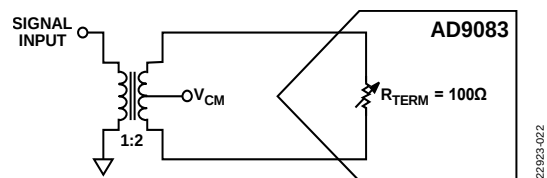
Figure 59. DC-Coupled Inputs to the AD9083 Using a Transformer (Note the Center Tap Connection Providing the Common-Mode Voltage)
