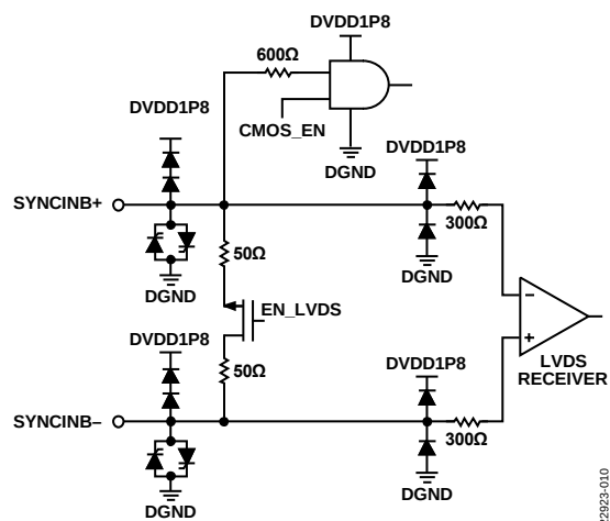
Figure 53. SYNCINB± Input
