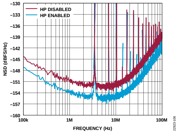
Figure 10. ADC NSD with and Without EN_HP, 1 GSPS
