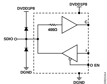
Figure 50. SDIO Input/Output
