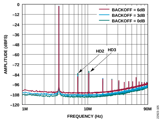
Figure 9. HD2 and HD3 at Various Backoff Values, 2 GSPS
