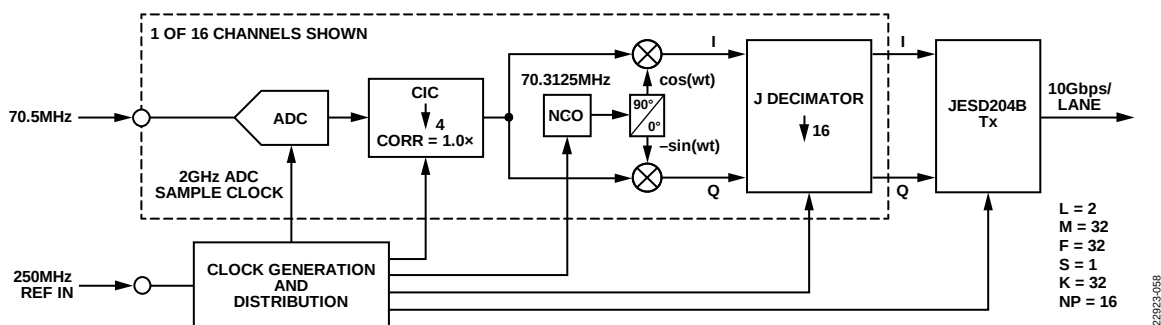
Figure 92. Narrow Bandwidth Complex Output Mode Block Diagram
