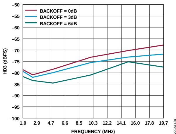
Figure 24. ADC HD3 vs. Frequency at Various Backoff Values and A_{IN} = -2 dB, 1 GSPS
