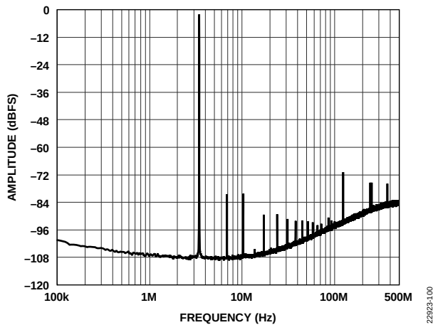
Figure 4. ADC Noise Floor at Backoff = 3 dB, 1 GSPS
