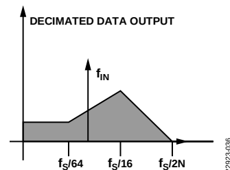
Figure 72. Frequency Spectrum of the Decimator Output
