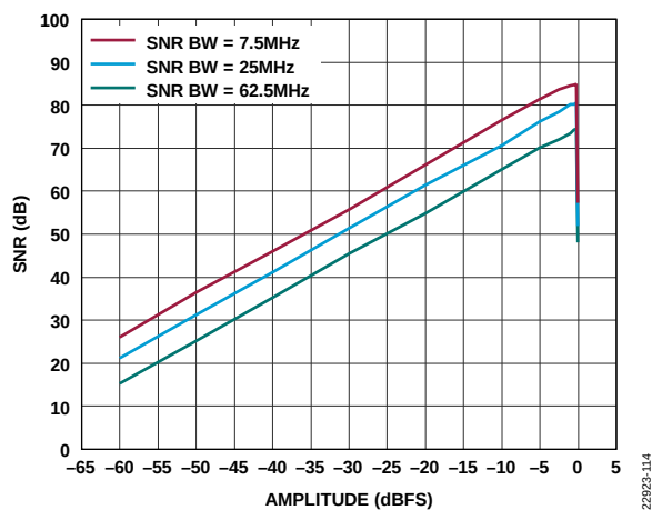
Figure 18. ADC SNR vs. Input Amplitude, 1 GSPS
