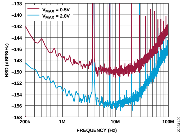
Figure 13. ADC NSD at Minimum and Maximum V_{MAX} Values, 2 GSPS
