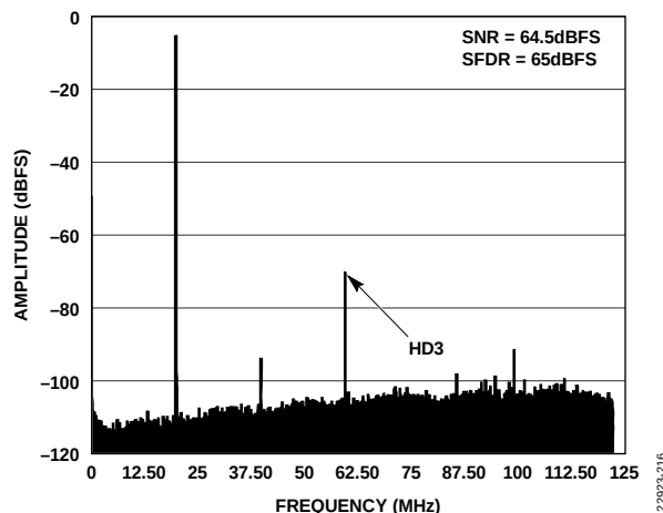
Figure 89. FFT Wide Bandwidth Real Output Mode
