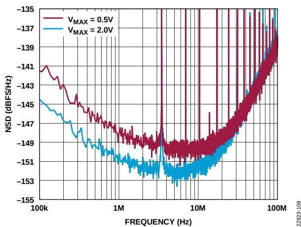
Figure 12. ADC NSD at Minimum and Maximum V_{MAX} Values, 1 GSPS
