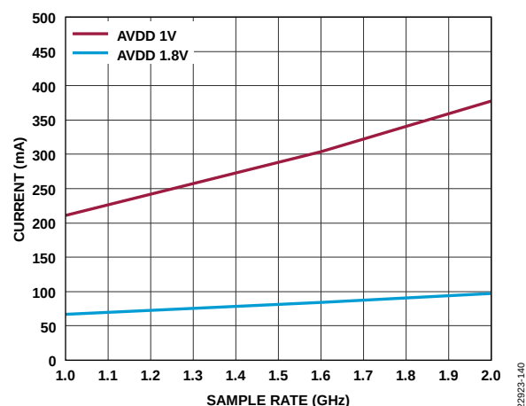
Figure 33. Supply Current vs. Sample Rate (Digital Domain Currents Vary with the DSP and JESD204B Setup)
