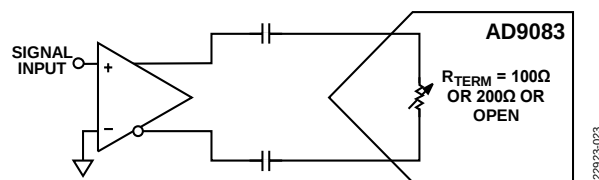
Figure 60. AC-Coupled Inputs to the AD9083 Using an Amplifier
