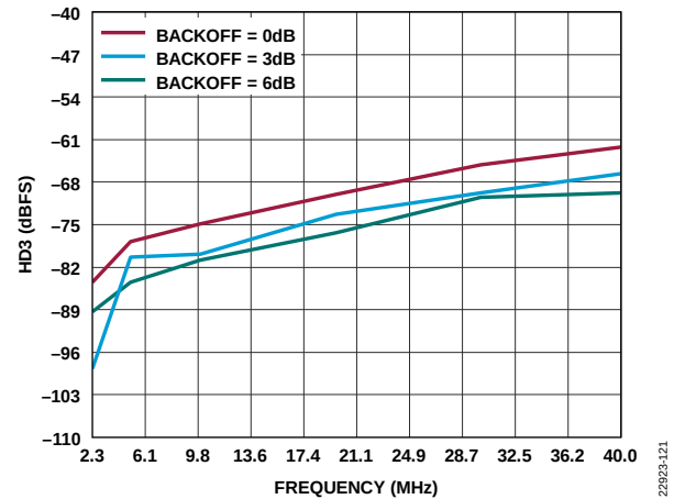
Figure 25. ADC HD3 vs. Frequency at Various Backoff Values and A_{IN} = -2 dB, 2 GSPS
