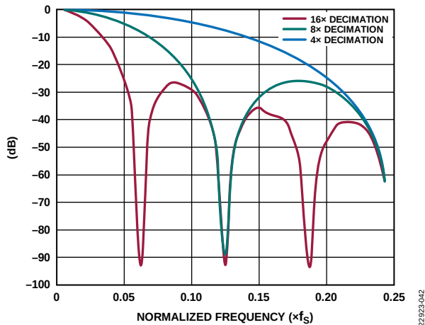
Figure 78. CIC Filter Response for Decimation Ratio = 4×, 8×, and 16×; Normalized to f_s
