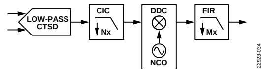
Figure 70. Simplified Diagram of the Digital Functional Block
