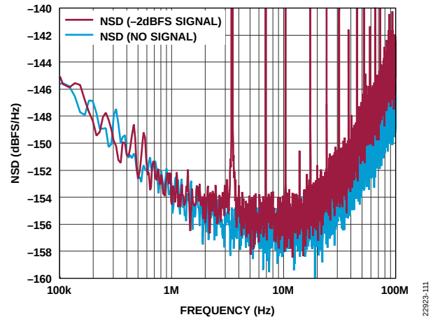
Figure 15. ADC NSD with and Without Full-Scale Input Signal, 2 GSPS
