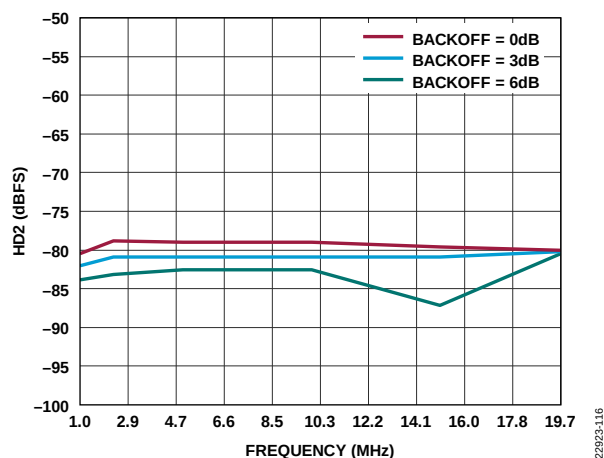
Figure 20. ADC HD2 vs. Frequency at Various Backoff Values and A_{IN} = -2 dB, 1 GSPS
