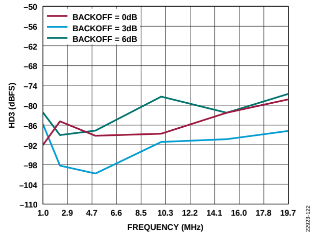
Figure 26. ADC HD3 vs. Frequency at Various Backoff Values and A_{IN} = -10 dB, 1 GSPS
