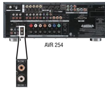
Figure 40 – Surround Back/Multiroom Preamp Outputs
