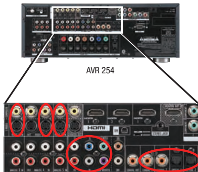
Figure 23 — Connecting a Composite- or S-Video-Equipped Disc Player
