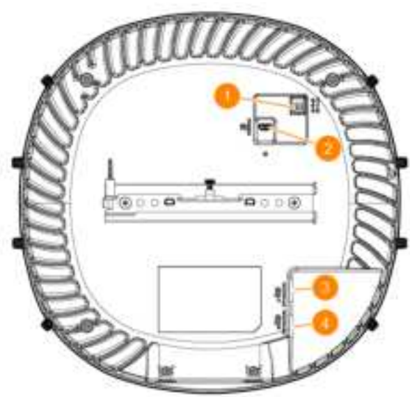
Figure 8 AP-754 Access Point Rear View
