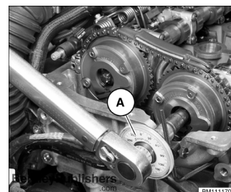
Detailed engine service, including VANOS camshaft timing adjustment. 117 Camshaft Timing Chain
