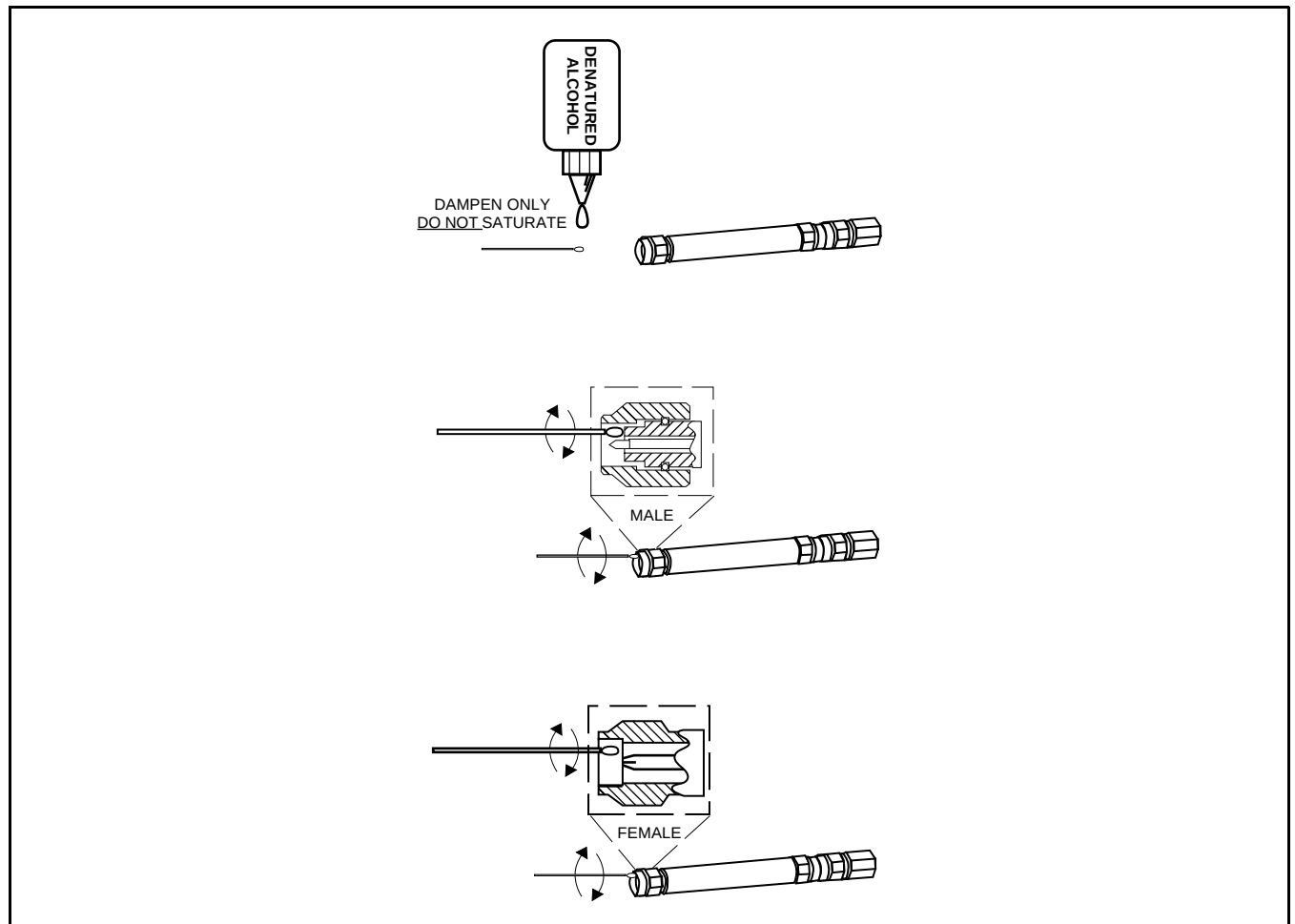
Figure 5. Cleaning Male and Female Connectors
