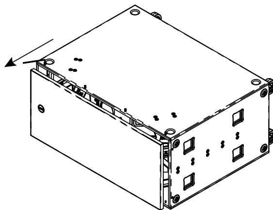
Figure 6.5: Grille removal
