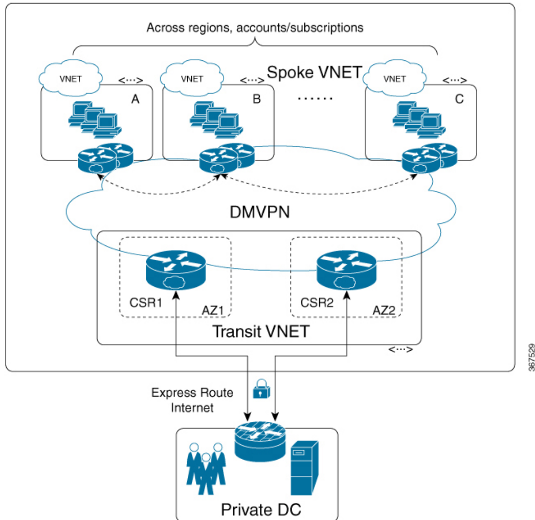
Figure 4: DMVPN all-CSR based Transit VNet Supported on Azure
