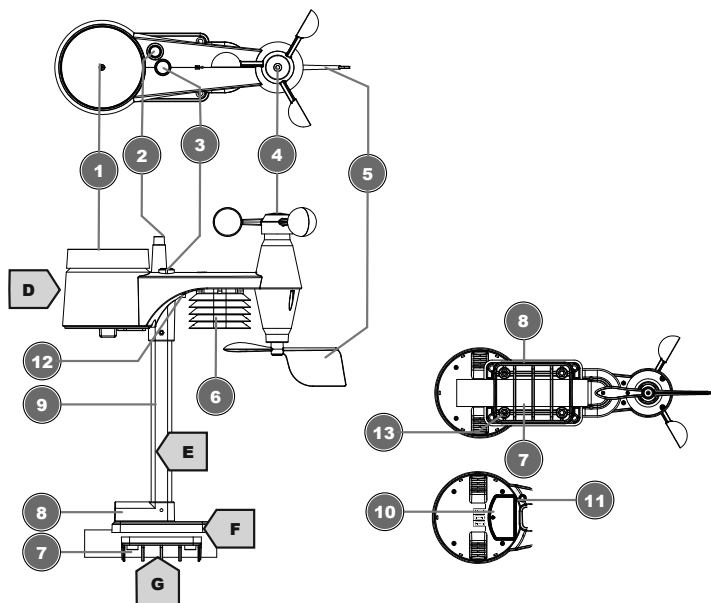
Illustration 2: All parts of the multisensor
